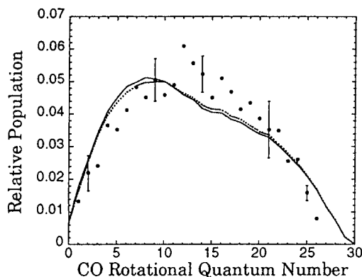
Figure 3. Comparison of two CPST predictions at 1720 \text{ cm}^{-1} based on different models of the ^1\text{CH}_2 distributions. The closed circles are the experimental points. Sample 1\sigma error bars are given. The solid line is the resultant distribution when the ^1\text{CH}_2 rotational population is approximated by the Boltzmann distribution which best fits the data. 17 The population is cut to zero for any ^1\text{CH}_2 state whose term value is greater than the available energy. The dotted line is the resultant distribution when that Boltzmann distribution is truncated at 80% of the available energy.
